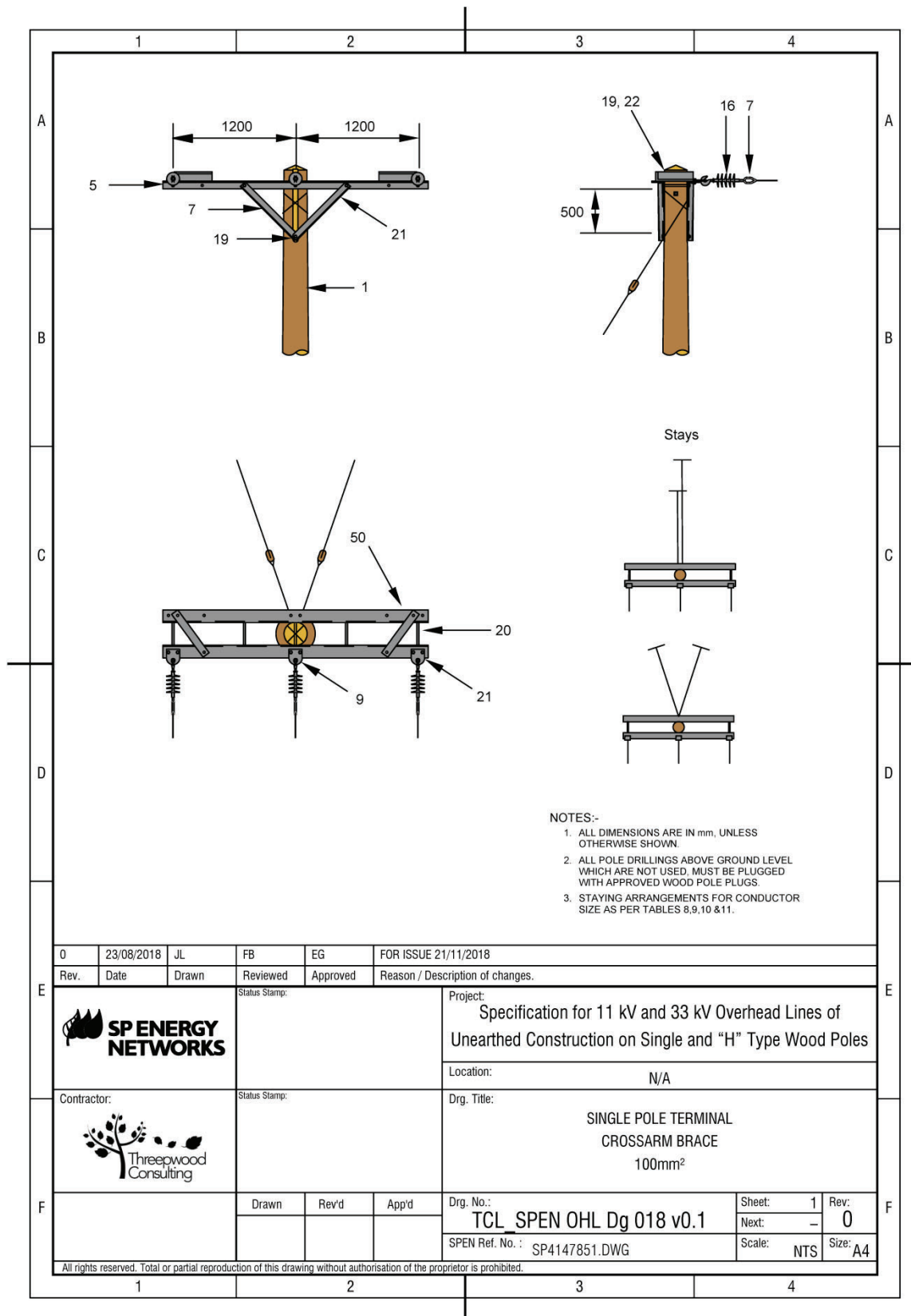
22.18 Figure 18 General Arrangement Single Pole Terminal Crossarm Brace 100mm 2 (Drawing No. SP4147851)
